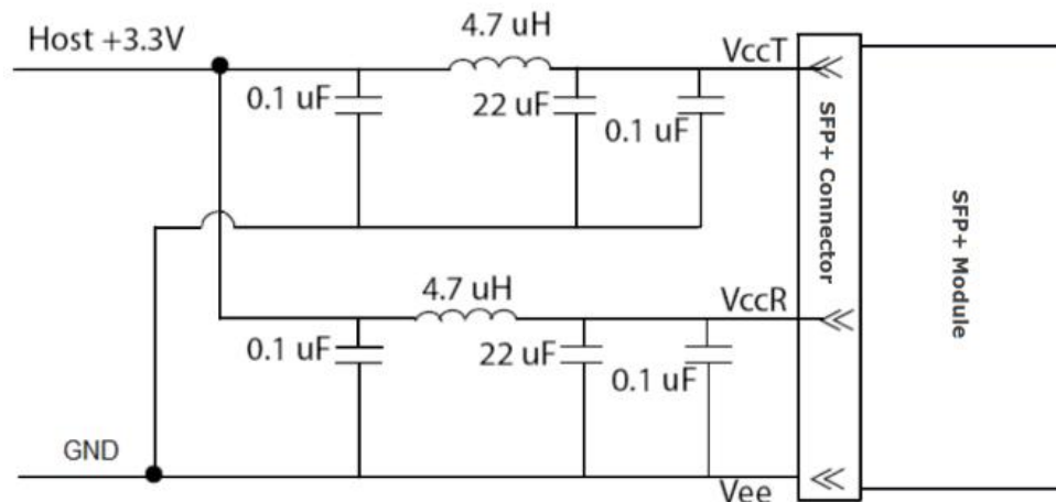
Figure 3, Recommended Host Board Power Supply Circuit
