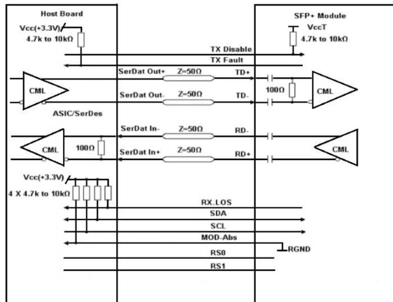
Figure 4, Recommended Interface Circuit
