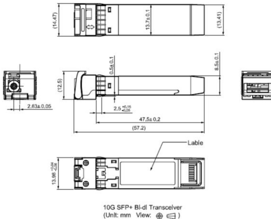
Figure 5, Mechanical Dimensions
