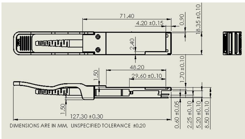
Figure 6. Mechanical Outline
