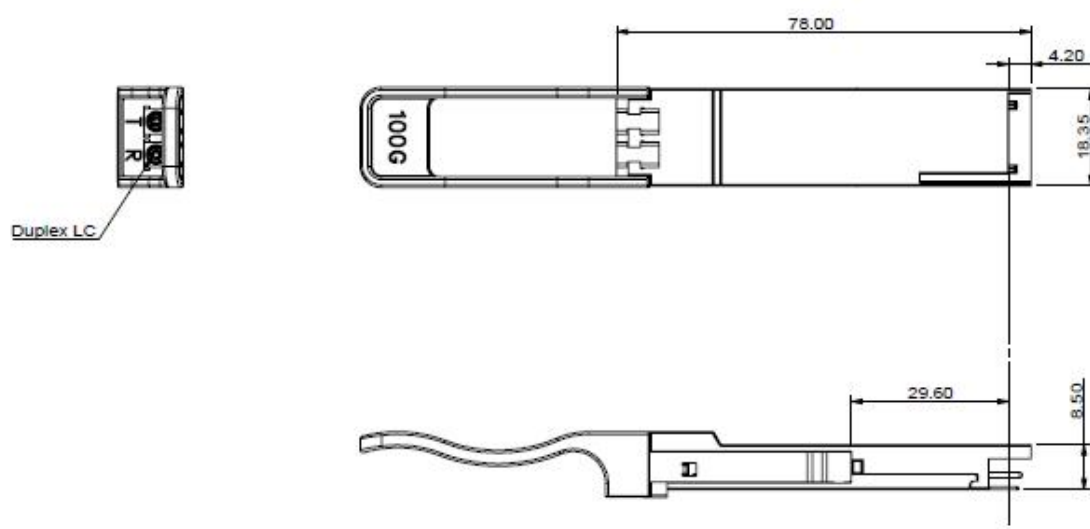
Figure 5. Mechanical Outline
